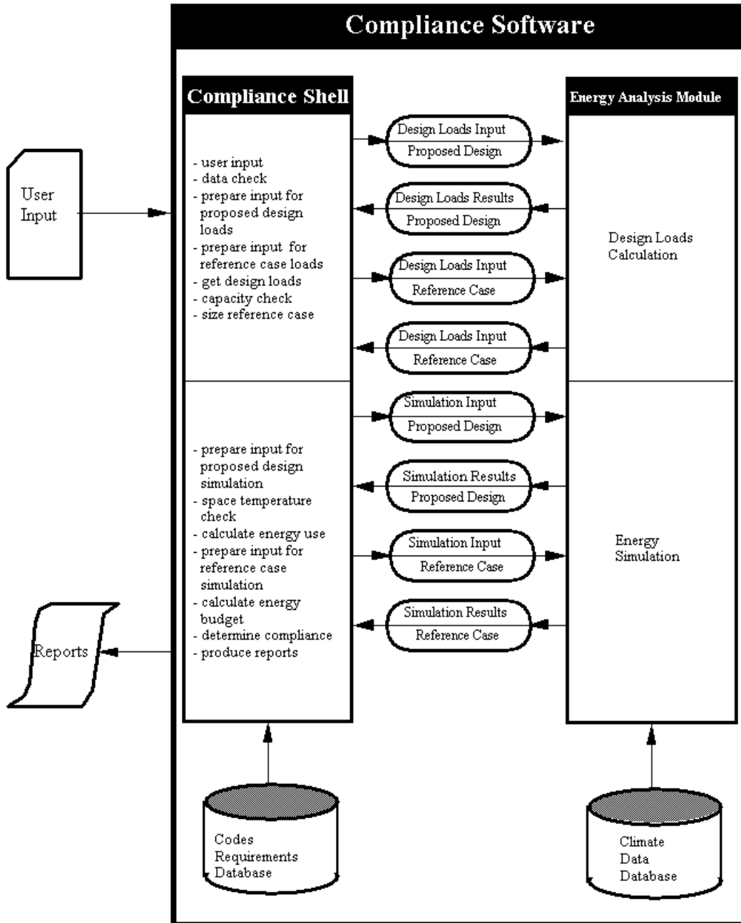
Figure 3.2.A. Software Structure 1
