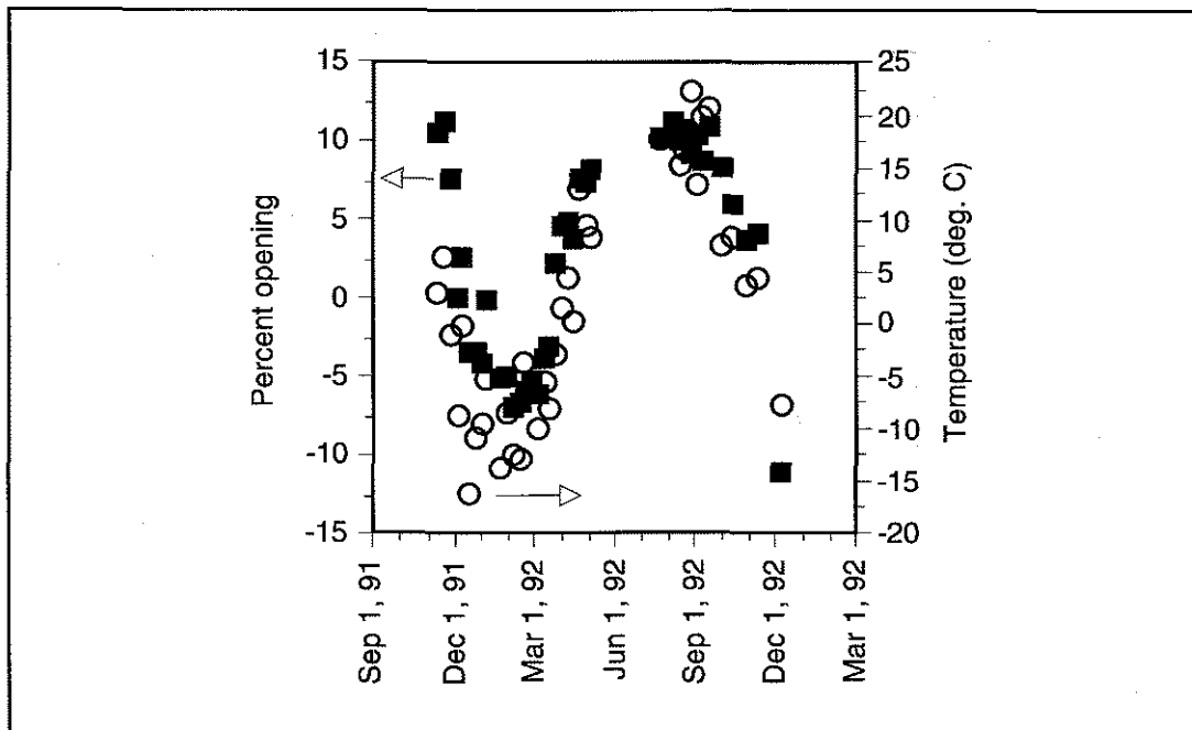
Figure 11. Comparison of the average rout width and temperature as measured in Montreal over one year. Pavements have a concrete base with an asphalt overlay. As a result, the response of the pavement to temperature variation is slow, and crack width varies accordingly. Crack width correlates weakly with average daily temperature but correlates strongly with the average temperature over four days.
