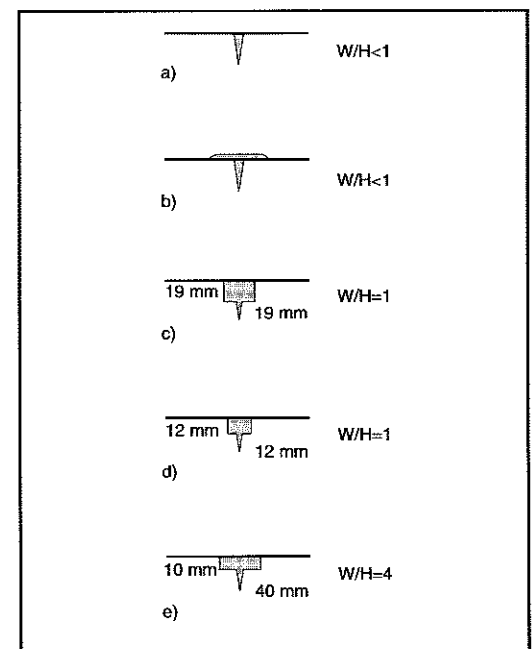
Figure 2. Crack geometries with (c-e) and without (a, b) routing. A sealant with W/H < 1 and placed in an active crack is strained more than one with W/H \geq 1 .
