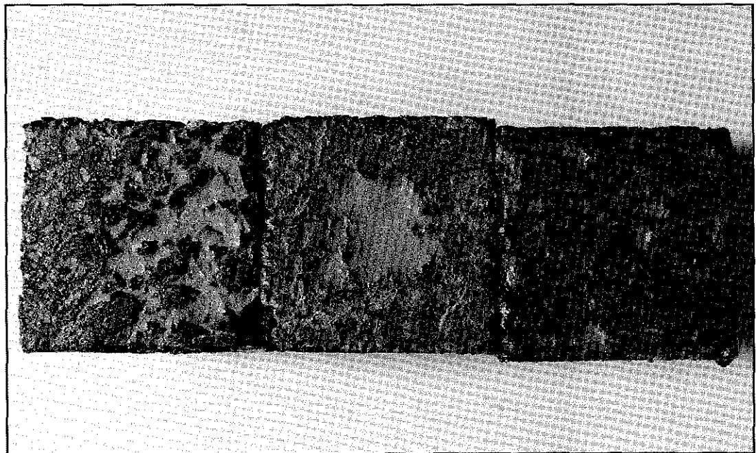
Figure 19. Surface of AC briquettes after tensile tests on sealant-briquette assemblies when the briquette is untreated (middle) and overheated (left). On the right, is the briquette surface without sealant. The briquettes were covered with dyed paste to increase the contrast between the holes in the briquette and the unaltered surface. On the untreated briquette, the sealant pulls out aggregates from the surface, leaving a hole in the middle of the briquette. On the overheated surface, there is no hole where the sealant was adhering. Instead, small holes are scattered across the surface where the hot-air lance caused damage.
