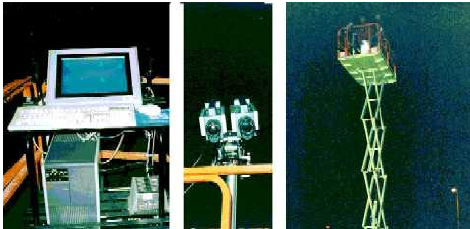
Infrared imaging system used at the experimental leak site. Shown are the PC-based control unit, dual-wavelength infrared cameras, and lift used to elevate infrared system 10 m above ground surface.
