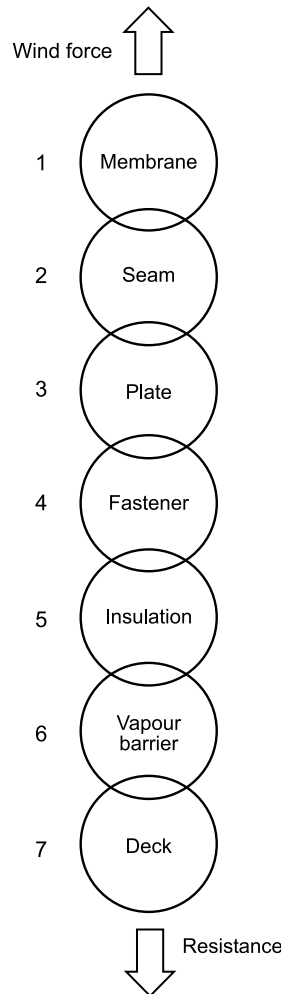
Figure 3. Force-resistance link diagram of single-ply roofs
